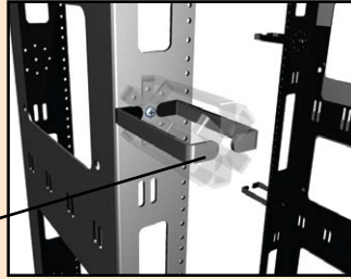
Eight (8) cable rings (2.5" x 4") allow for rotational mounting
