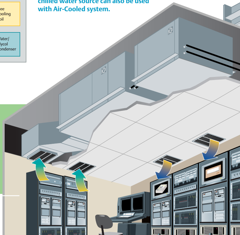
The components in units are located for easy service (1 ton self-contained unit shown)
