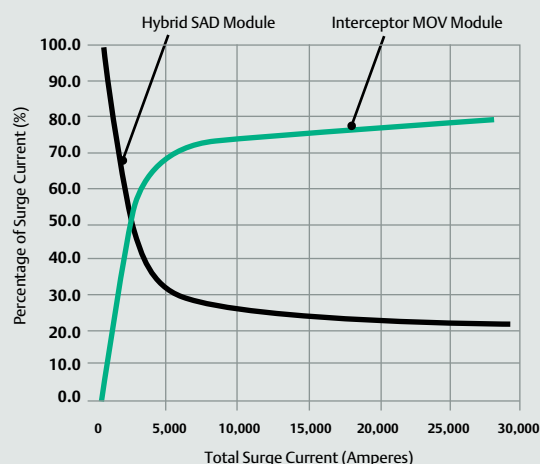
Typical Hybrid Advantage Surge Current Sharing Data
